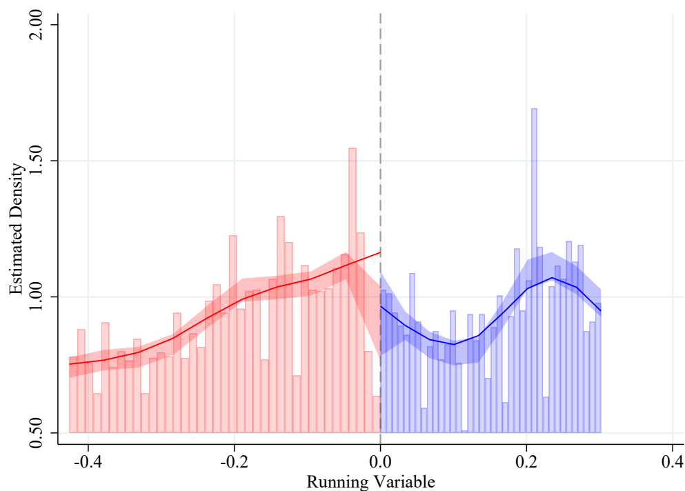
Figure J.12: Histogram and Estimated Density of the Running Variable
